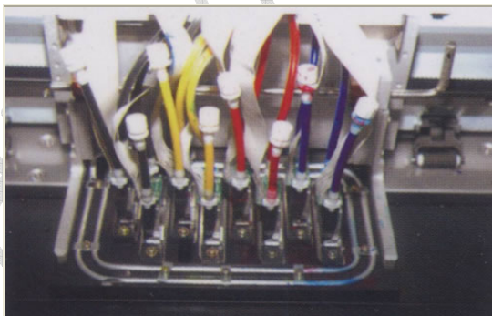
Print head Fixing
